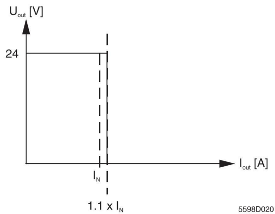
Figure 3-27 U/I characteristic
