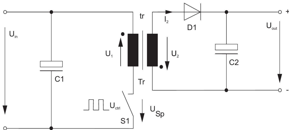
Figure 2-13 Flyback converter with switch S1 opened
