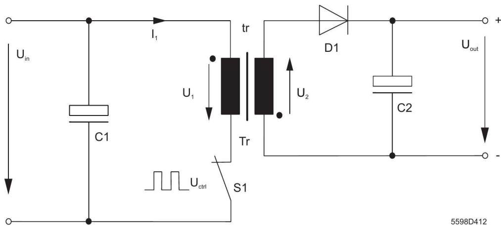
Figure 2-12 Flyback converter with switch S1 closed
